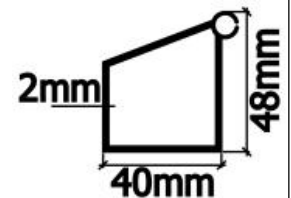
Eave purlin
